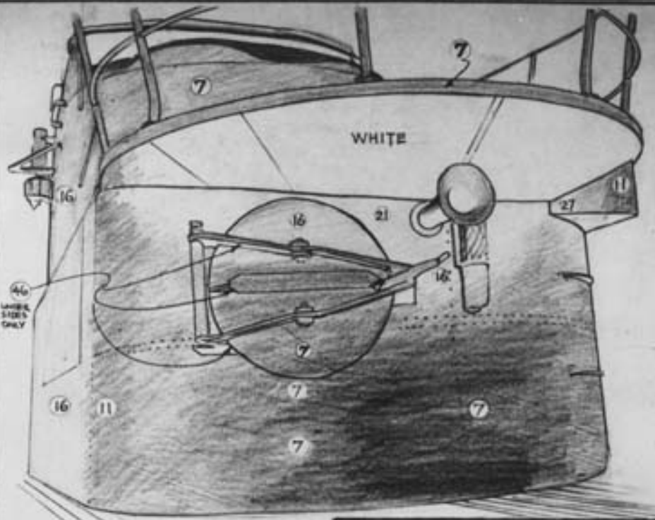
DETAIL NO. 8 BOW
