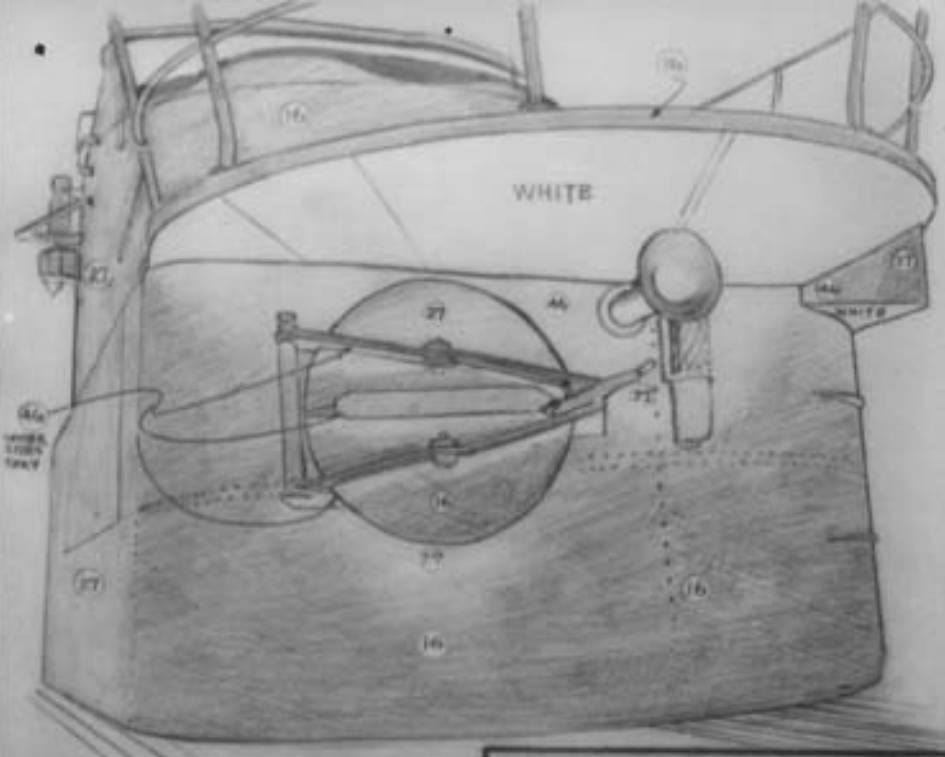
DETAIL NO. 8 BOW
